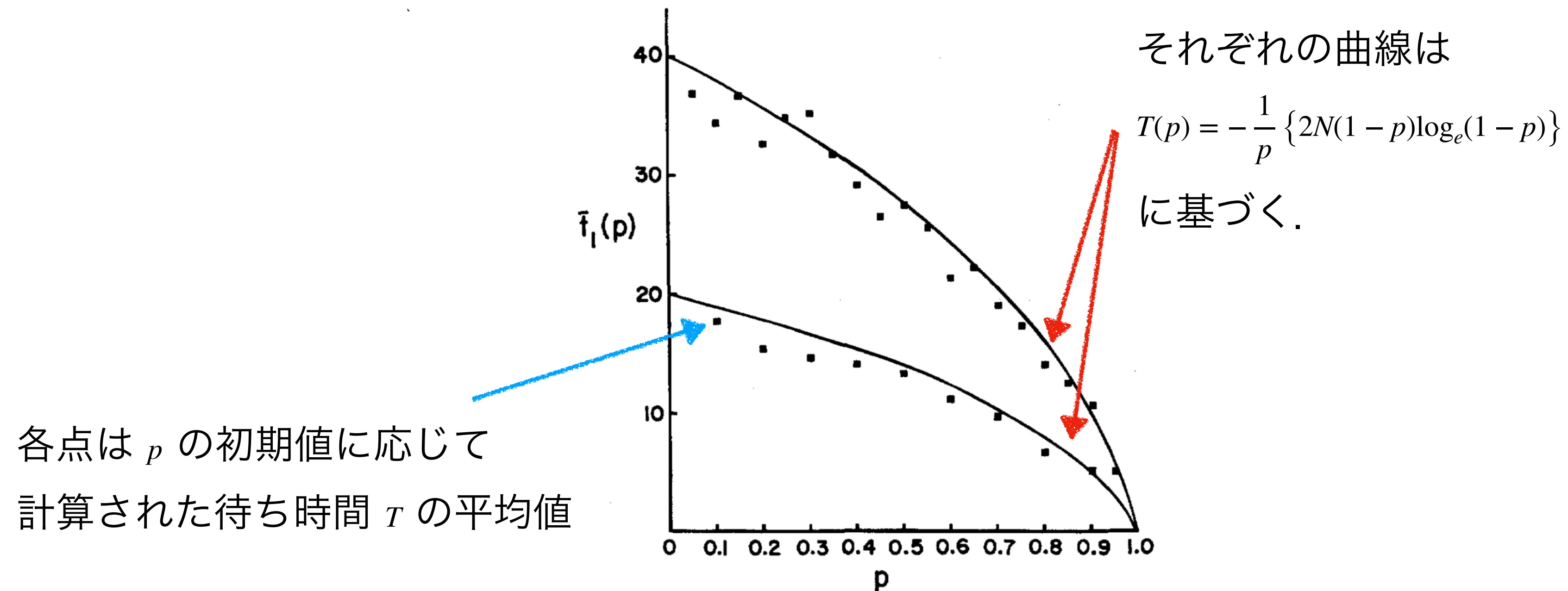
FIGURE 1.—Average number of generations until fixation of a selectively neutral mutant gene as a function of its initial frequency. The theoretical values are represented by curves and those of Monte Carlo simulation by dots. 2N_e=20 in the upper curve and 2N_e=10 in the lower one.
