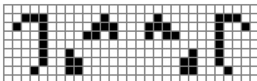
Puffer 1
