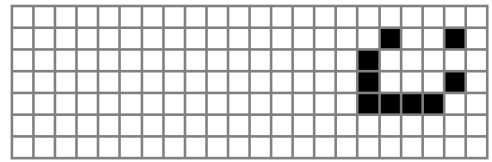
Lightweight spaceship
